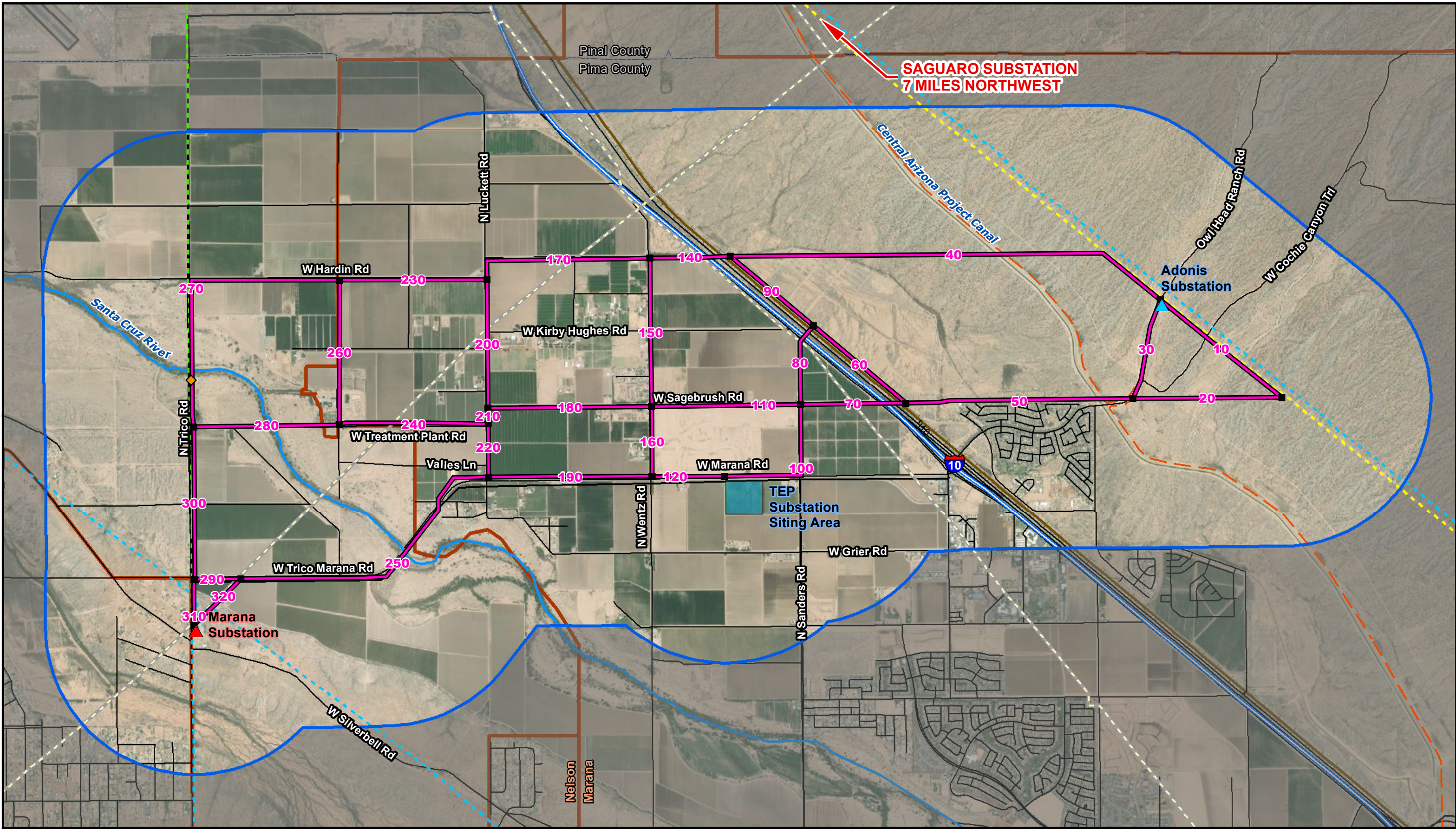
Figure 4 Preliminary Route Segments Saguardo - Marana 115kV Transmission Line Project Arizona G&T Cooperatives Draft - Not for Construction
